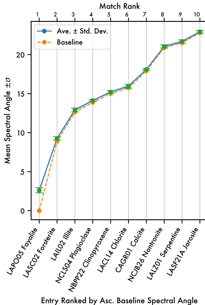
LAPO05 Fayalite Mean Spectral Angle Match
